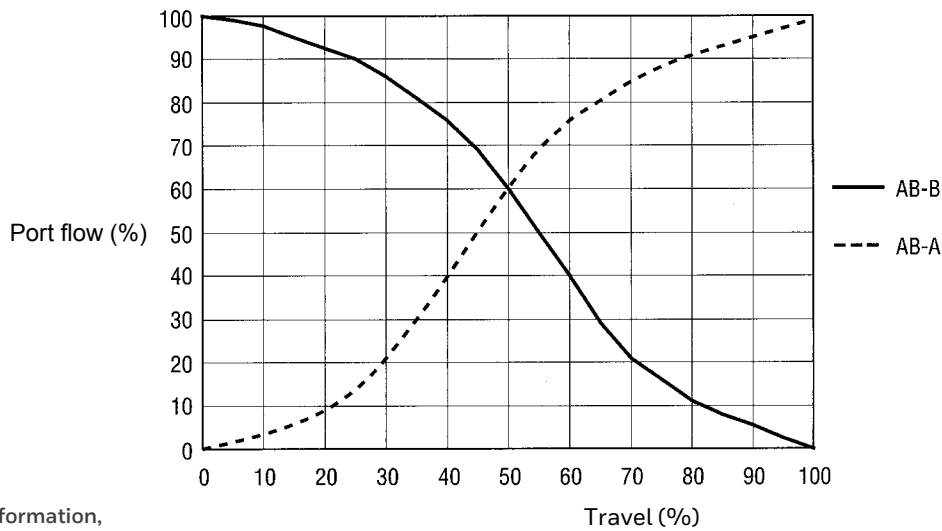
Fig. 10. Typical 3-way valve diverting characteristic at constant pressure on port AB
