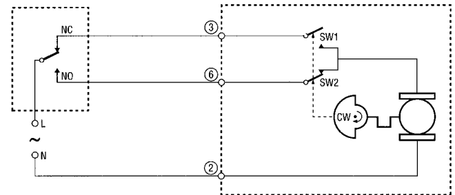
Fig. 3. Logic sequence diagram with 3-wire actuator for SPDT controller
